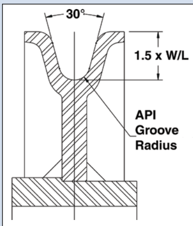
TYPICAL API SHEAVE RIM PROFILE
